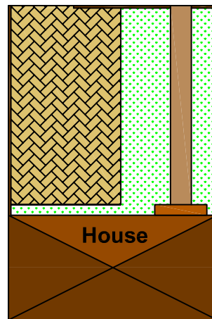
Permeable paving which allows rain water to drain through to sub grade
