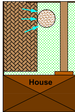
No-permeable paving with a rain garden to soak away water run off from hard standing
