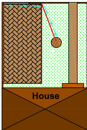
No-permeable paving with aco channel to front edge which drains into soak away
