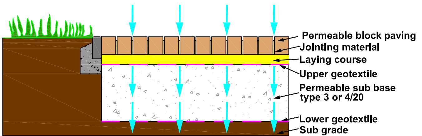
Permeable paving - cross section
